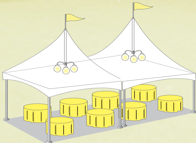
Interior layout of a 20 x 40 frame tent with 8-tables, 2-light units and no center poles.
