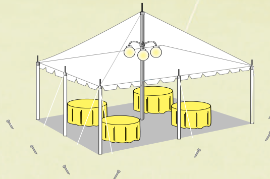
Interior layout of a 20 x 20 pole tent with 4-tables, 1-light unit and 1-center pole.
